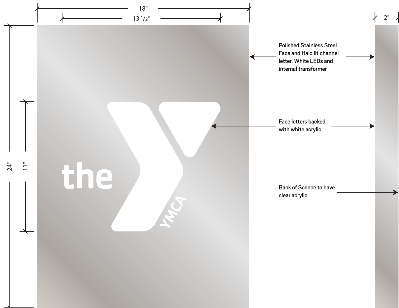
1 TYPICAL LAYOUT SCALE: 1:4 FONT - IMPORTED LOGO EACH TO HAVE INTERNAL TRANSFORMER
